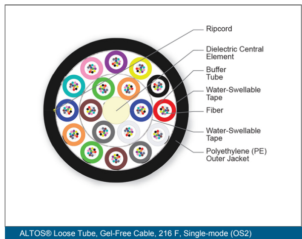
ALTOS® Loose Tube, Gel-Free Cable, 216 F, Single-mode (OS2)
